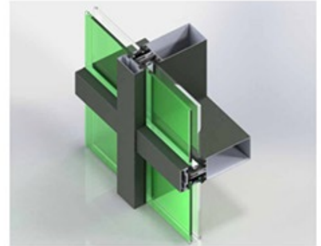
F50 Classic Capped Facade System
