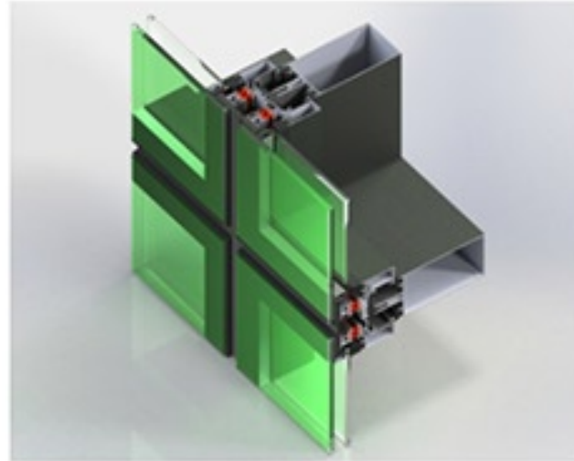
F50 Classic Silicone Facade System
