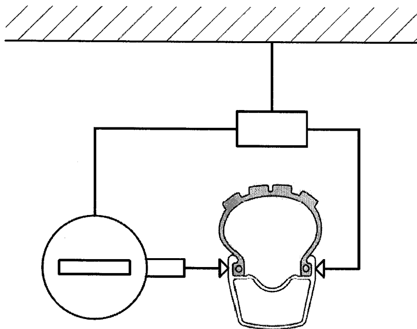
Figure 4 — Wheel laid down on tire and axle
