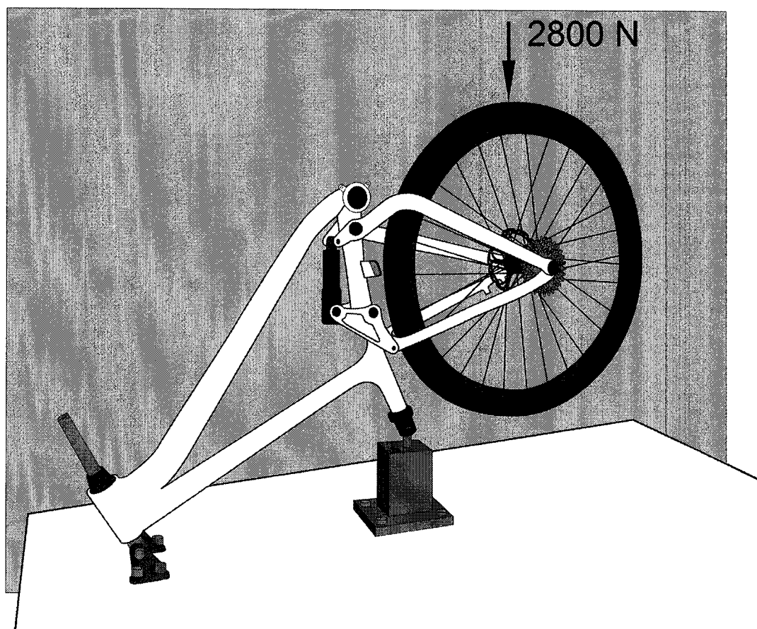
Figure C.1 — Examples of suspension frames — Tyre-clearance test
