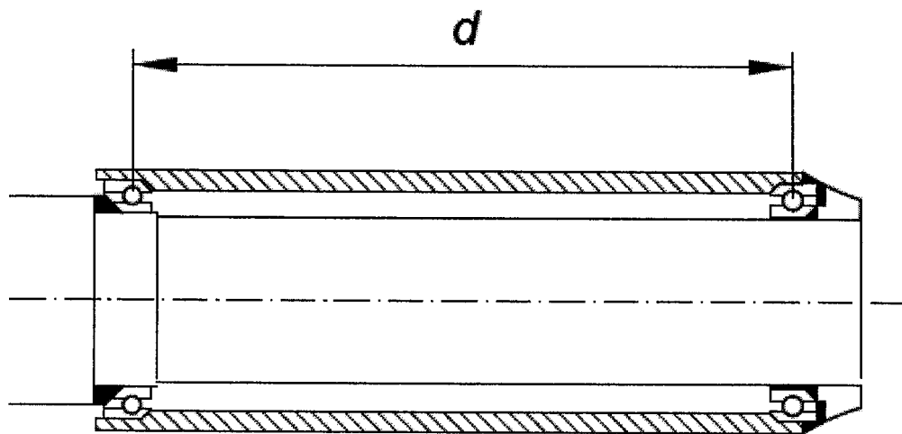
b) Measurement with integrated bearings
