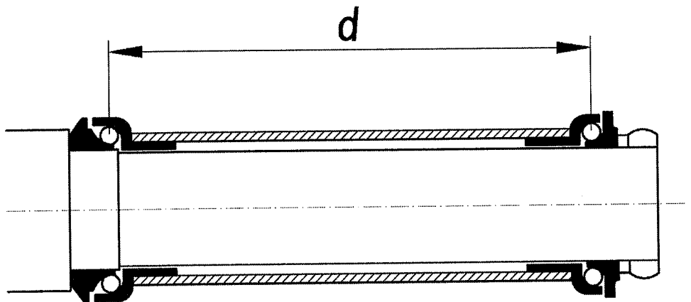
a) Measurement with external cup bearings
