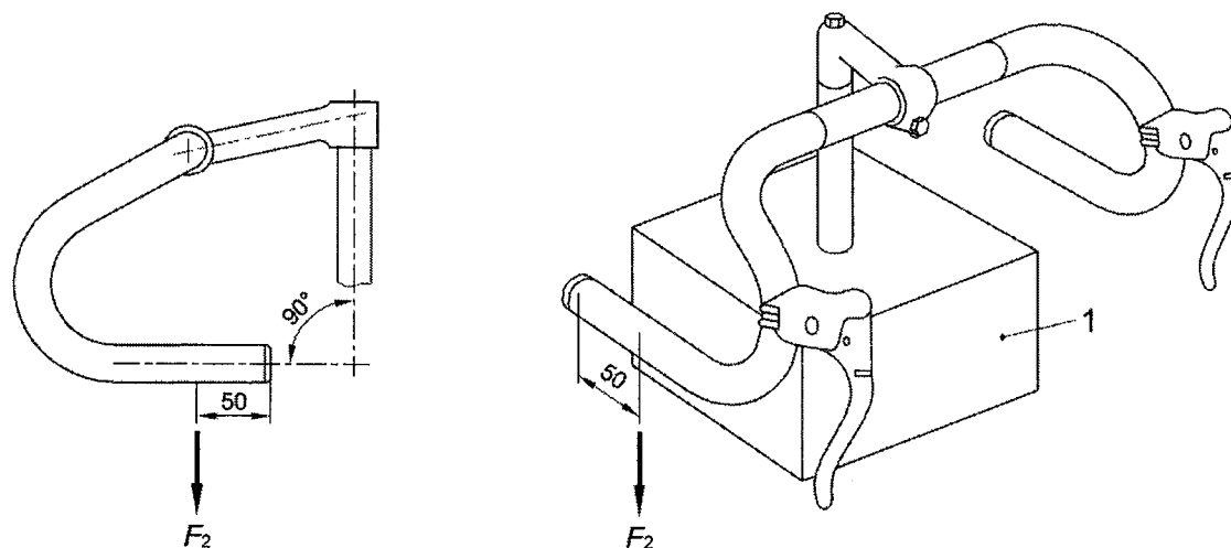
a) Orientation of adjustable handlebars
