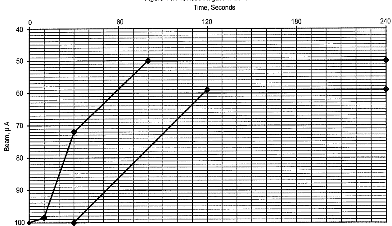
Figure 44.1 Flaming liquid fuel profile
