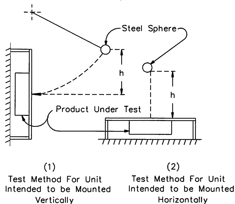
Figure 60.1 Jarring test
