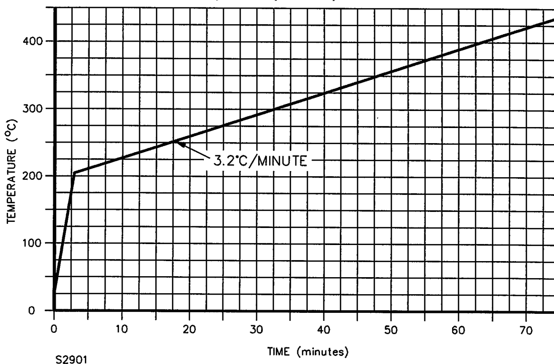
Figure 45.1 Hotplate temperature profile
