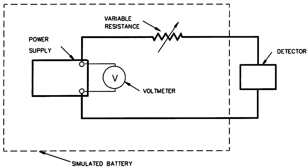
Figure 35.1 Test circuit
