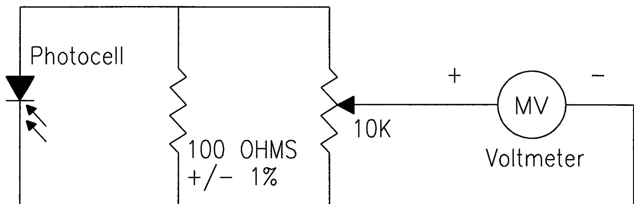
Figure 37.3 Potentiometer placement
