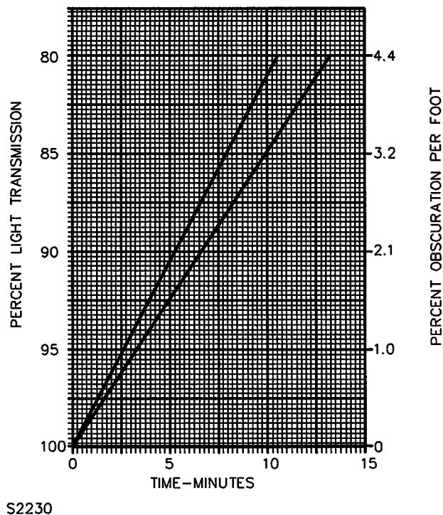
Figure 50.4 Smoke build-up rate – sensitivity test – 40°C ambient – aerosol – 32 fpm
