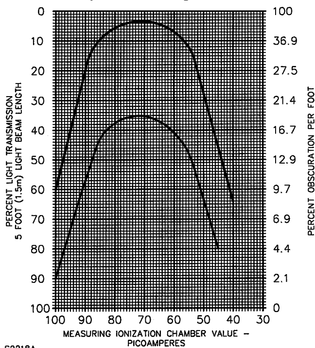
Figure 44.8 Paper fire – ceiling location
