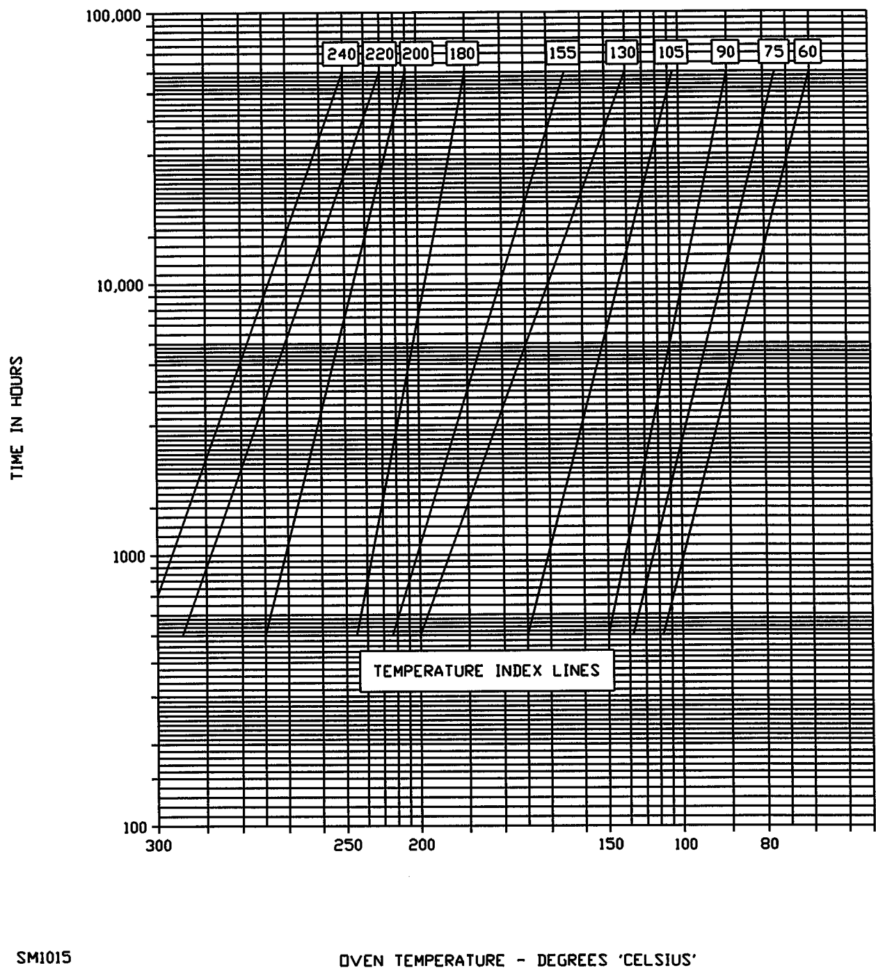
Figure 77.1 Aging time versus aging temperature
