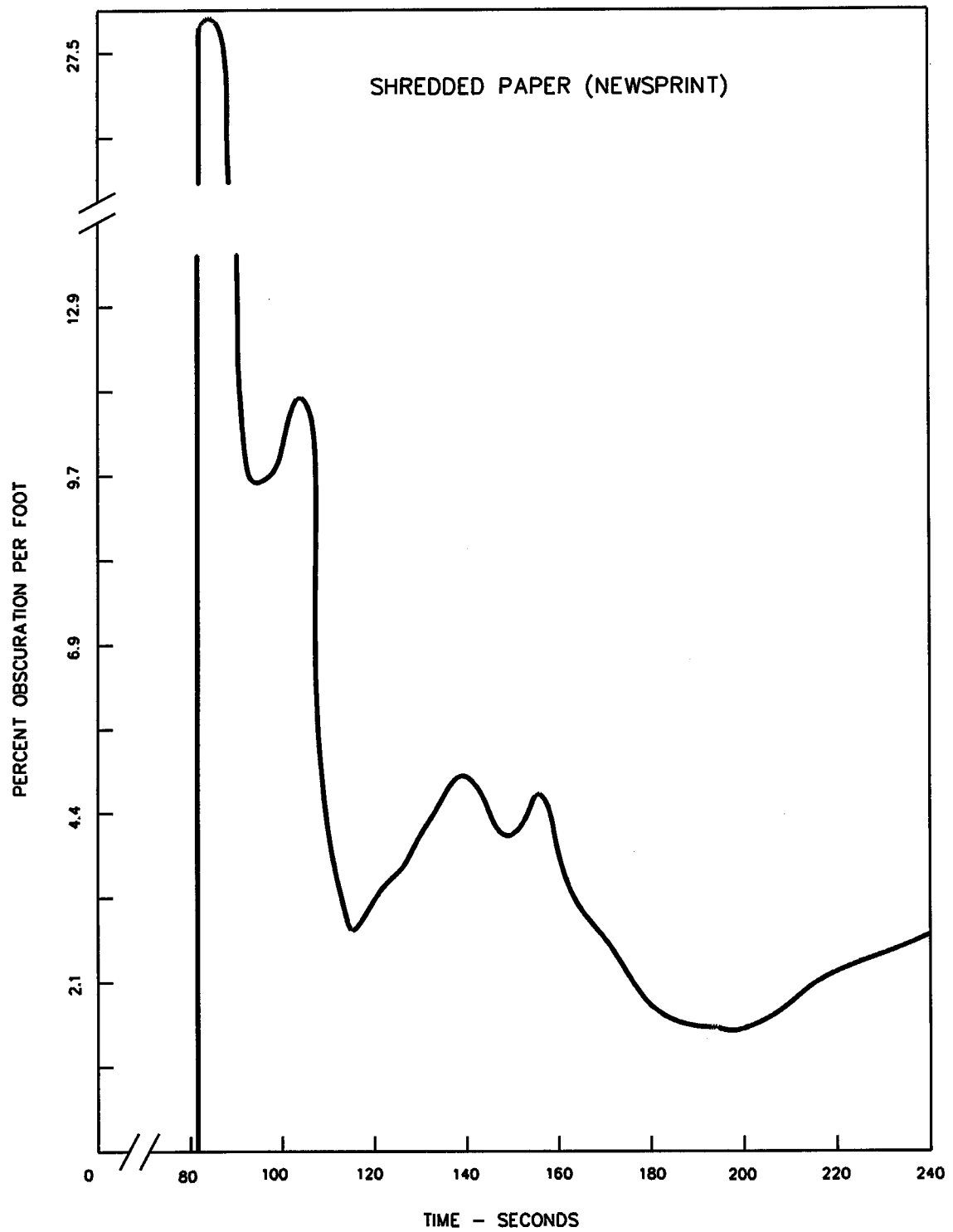
Figure 44.6 Shredded paper (newsprint) profile
