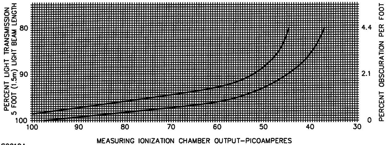
Figure 37.1 Sensitivity test limits – aerosol – 32 fpm
