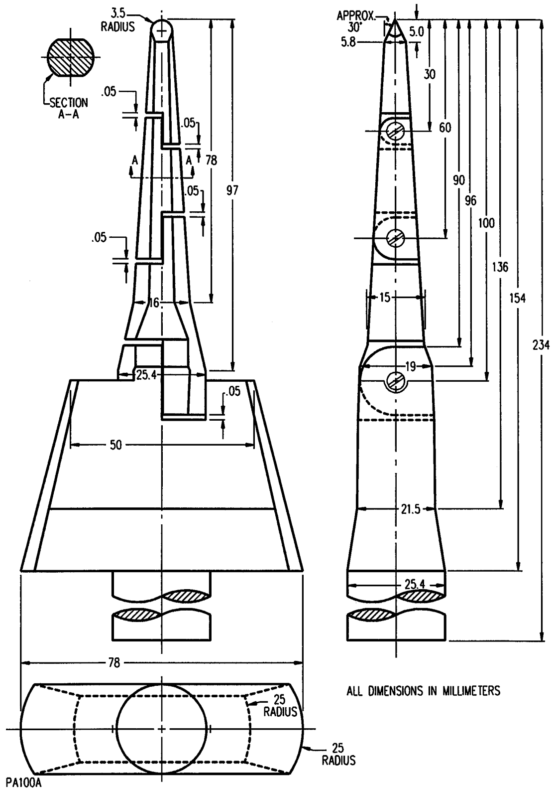
Figure 70.1 Articulated probe
