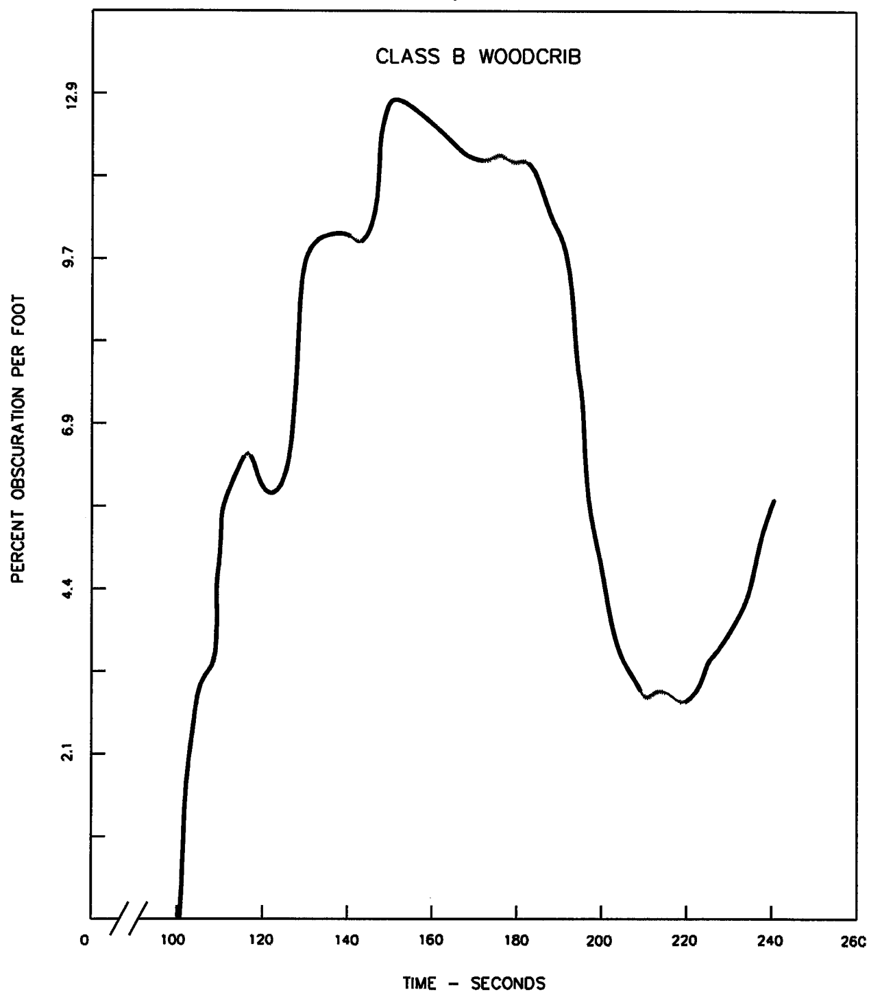
Figure 44.7 Woodcrib profile
