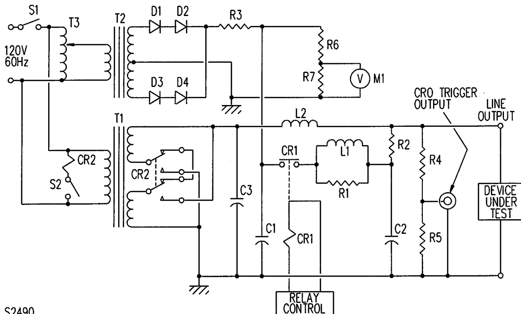
Figure 53.1 Surge generator circuit
